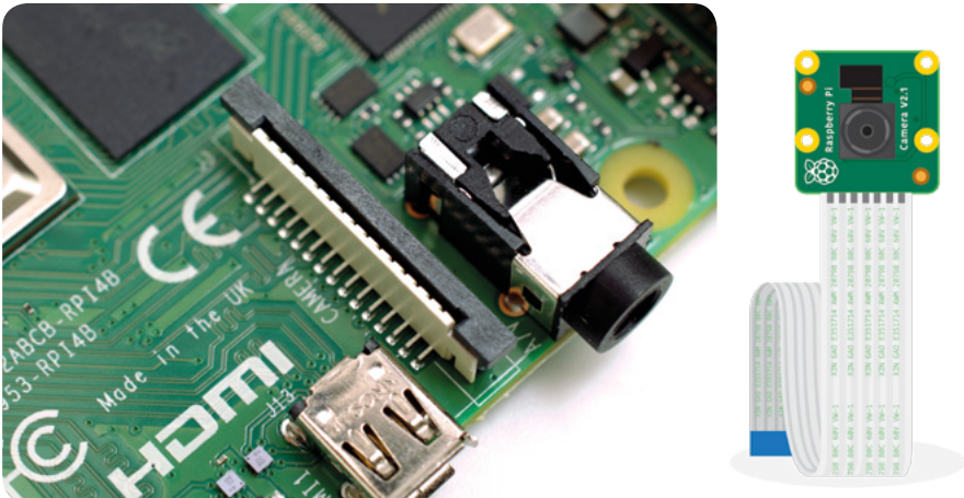
▲ Figure 1-9: Raspberry Pi's camera connector
