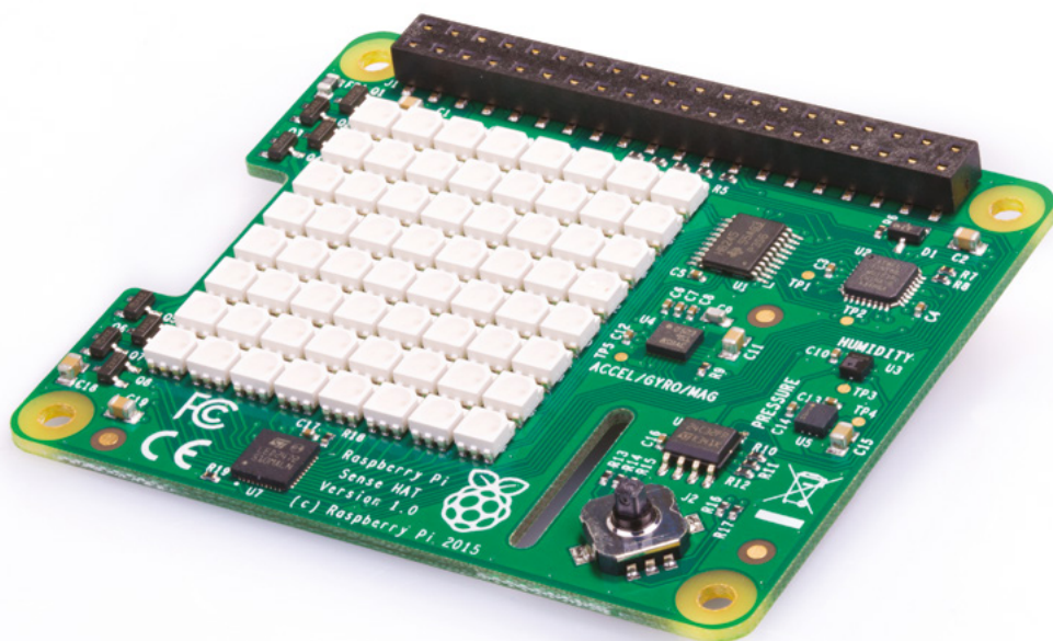
▲ Figure 1-16: The Sense HAT
