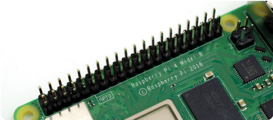
▲ Figure 1-14: Raspberry Pi's GPIO header
