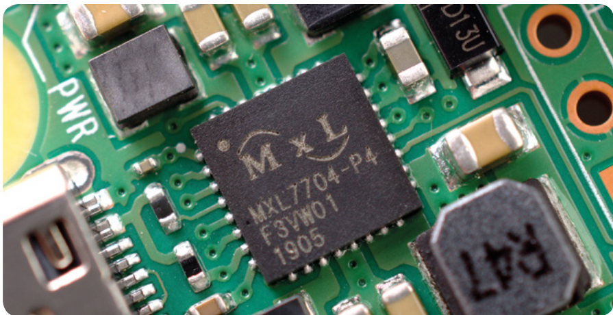
▲ Figure 1-5: Raspberry Pi's power management integrated circuit (PMIC)
